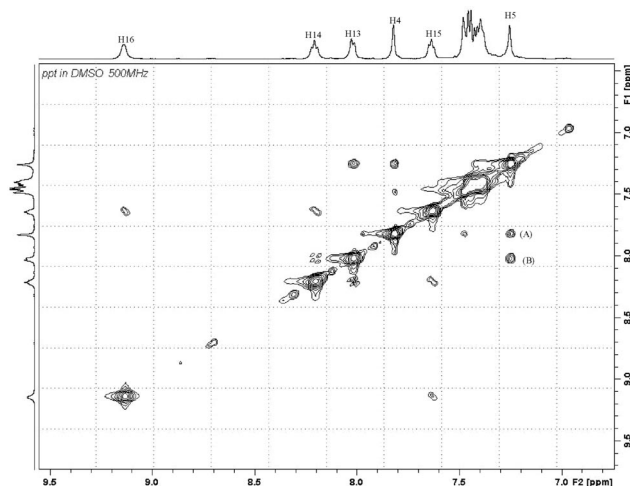
Figure 2. ROESY NMR of complex ( \pm )-4.
