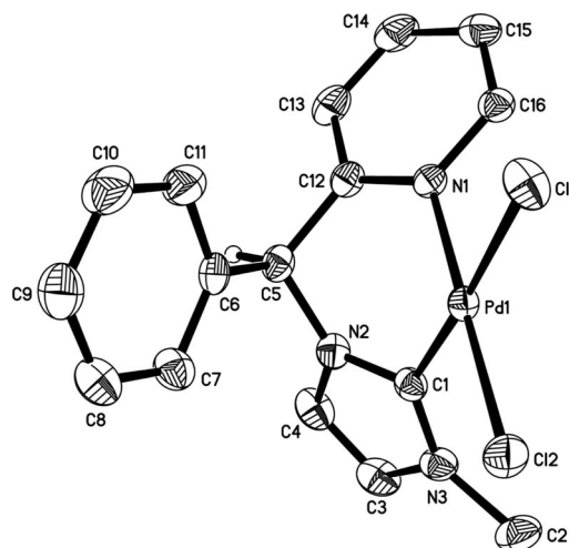
Figure 5. Molecular structure of complex ( S )- 4 .
