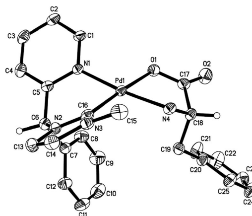
Figure 3. Molecular structure of complex ( R_C, S_C )-5.
