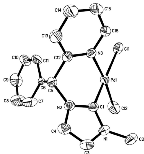
Figure 1. Molecular structure of complex ( \pm )- 4 .
