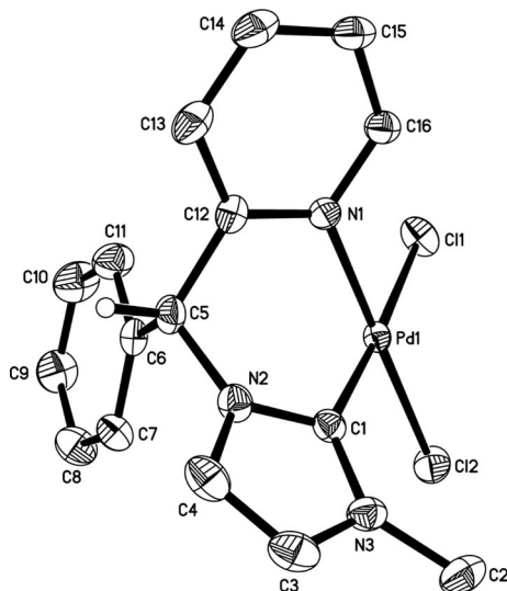
Figure 4. Molecular structure of complex ( R )- 4 .
